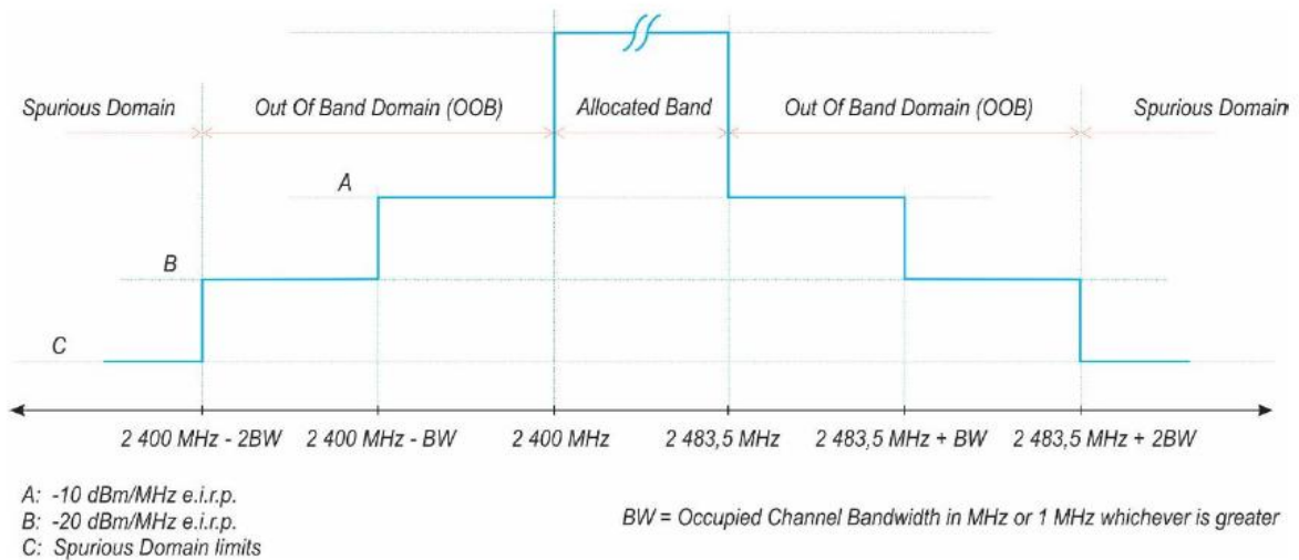
Figure 3: Transmit mask
